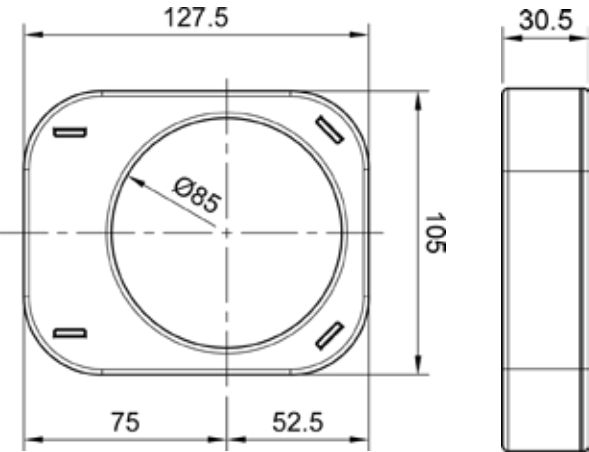
TECHNICAL SCHEMATA
